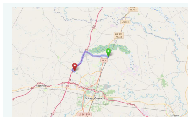
Figure 1: Tornado path through Rocky Mount, NC ( OpenStreetMap ).
