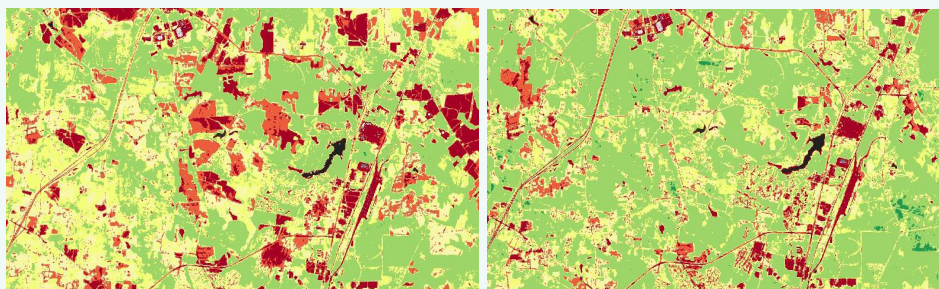
Figure 2: NDVI Composite Images of Rocky Mount, NC. The left panel shows pre-tornado conditions, while the right panel illustrates post-tornado conditions after the July 2023 EF-3 tornado.
