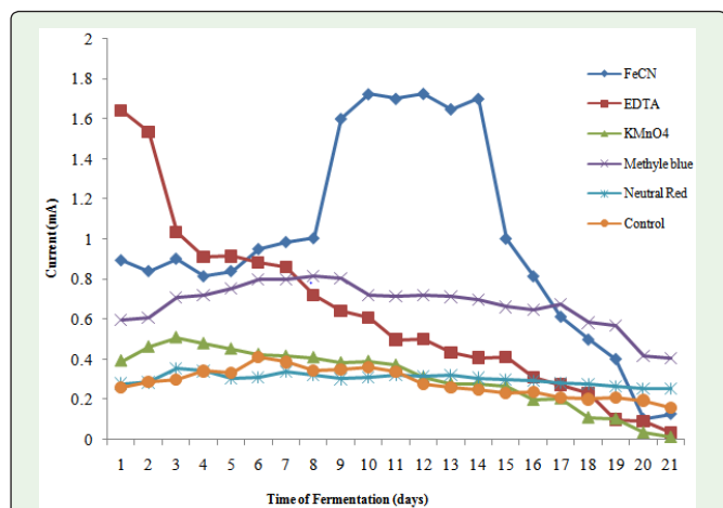
Figure 1: Current generated with exogenous mediators in MFC using kitchen waste as substrate.
