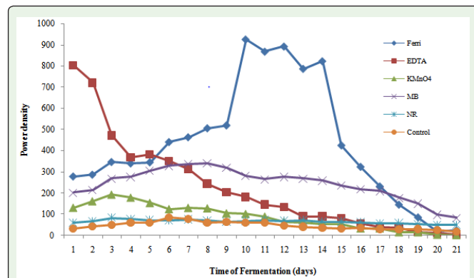
Figure 2: Power density generated with exogenous mediators in MFC using kitchen waste as substrate.
