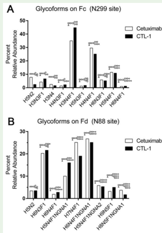
Figure 2: Relative abundance of glycoforms at each glycosylation site on cetuximab and CTL-1. Antibodies were IdeS cleaved and TCEP reduced to separate the major antibody subunits. Fc/2 and Fd regions were isolated and run by LC-MS to analyze glycoform heterogeneity at each glycosylation site. Peaks in the LC-MS chromatograms were correlated to their respective glycan structures based on previously published work on cetuximab glycoprofiles [18,21]. Sugar residues are N-acetylglucosamine (□), mannose (○), galactose (◇), N-glycolyl neuraminic acid (◊), and fucose (△). Glycan compositions are given in terms of hexose (H), N-acetylhexosamine (N), deoxyhexose (F), and N-glycolyl neuraminic acid (NGNA).
