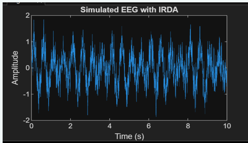
Figure 1: EEG signal wave chart, this figure would display the raw EEG signal in the time domain, highlighting the intermittent \delta activity.
