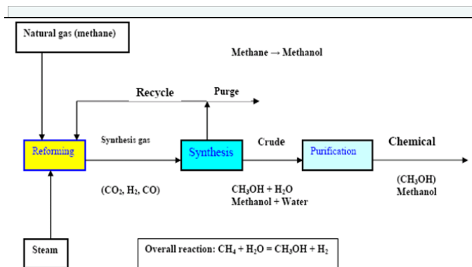
Figure 2 Schematic diagram shows methanol production (Omer, 2006).
