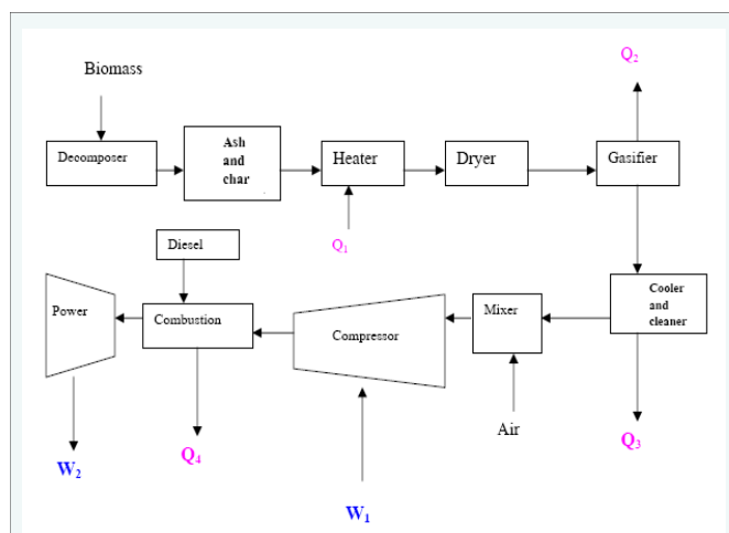
Figure 7 Advanced biomass power with diesel engine (Omer, 2006).
