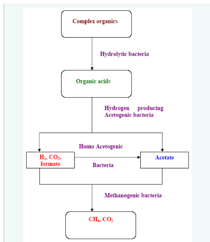
Figure 3 Biogas production process (Omer, 2003).
