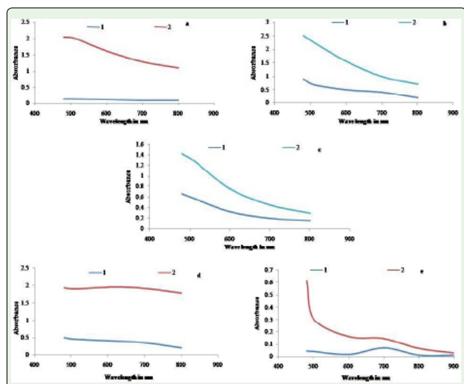
Figure 1: Micro-scan spectrum of fungal liquid (1) before and (2) after synthesis silver nanoparticles of C. tropicum , C. keratinophilum , F. oxysporum , A. niger and V. lecanii (a-e).
