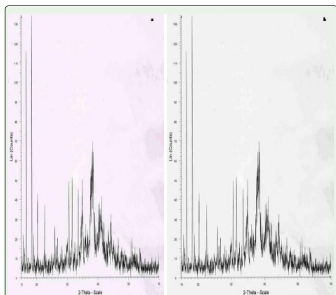
Figure 2: XRD pattern of biosynthesized silver nanoparticles (a) C. tropicum and C. keratinophilum (b) F. oxysporum , A. niger and V. lecanii .
